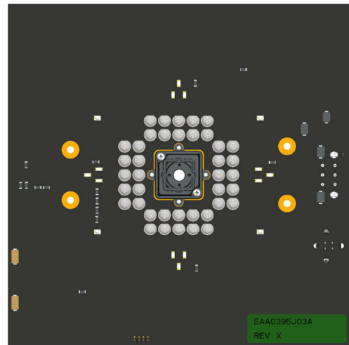
EAA0395J03A, vers. D - 2 Camera Systems
